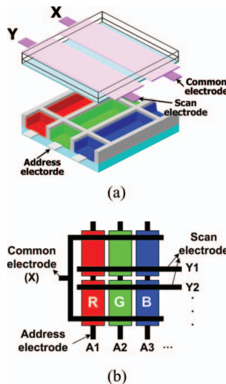
Figure 2. (a) Test panel structure and (b) schematic diagram of three electrodes in 42-in. HD PDP test panel employed in current study.
